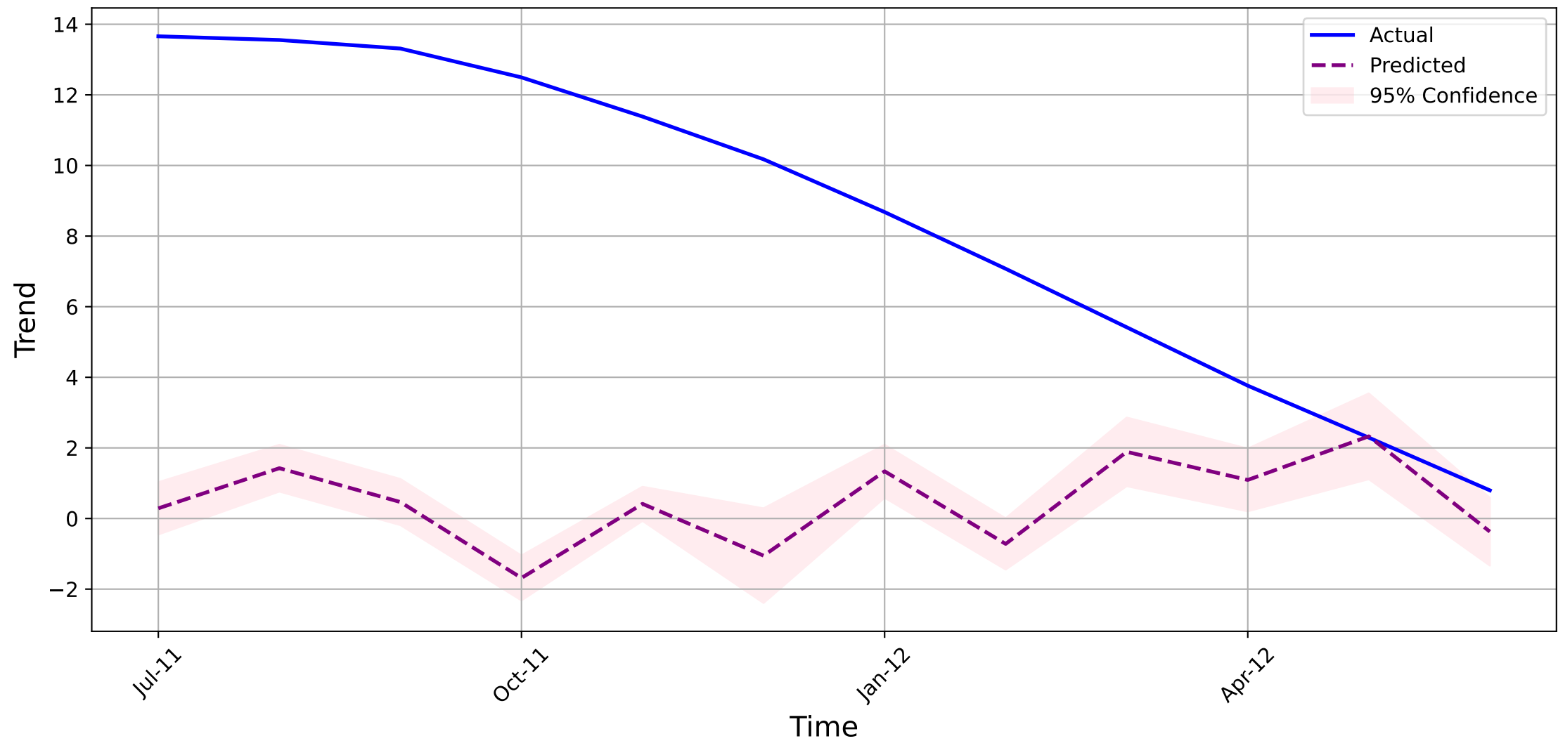
Disinformation/Misinformation-ALL - Validation
